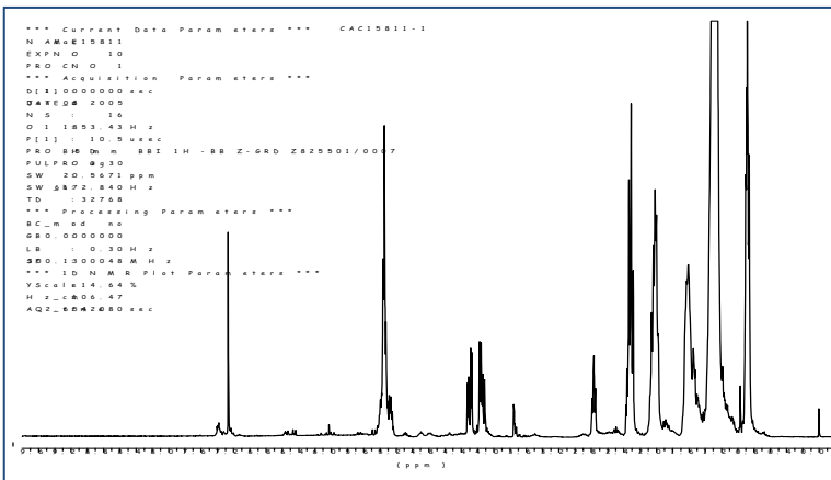
Figure 1 ^1\text{H-NMR} : Spectra Reference for Tamanu Oil (Pure Virgin) Identification
