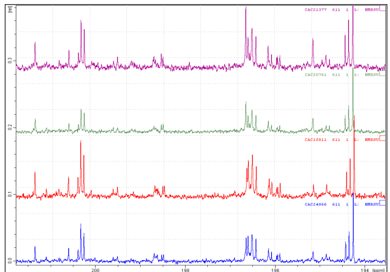
Figure 2 ^{13}\text{C-NMR} : Spectra Reference for Tamanu Oil (Pure Virgin) Identification
